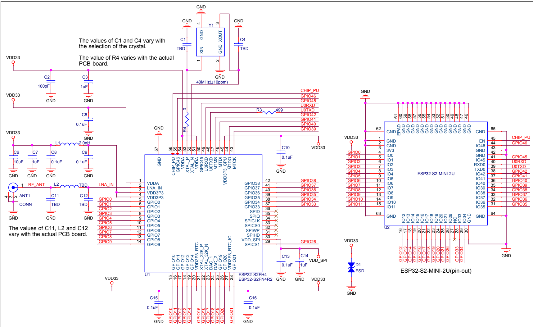
Figure 6: ESP32-S2-MINI-2U Schematics
