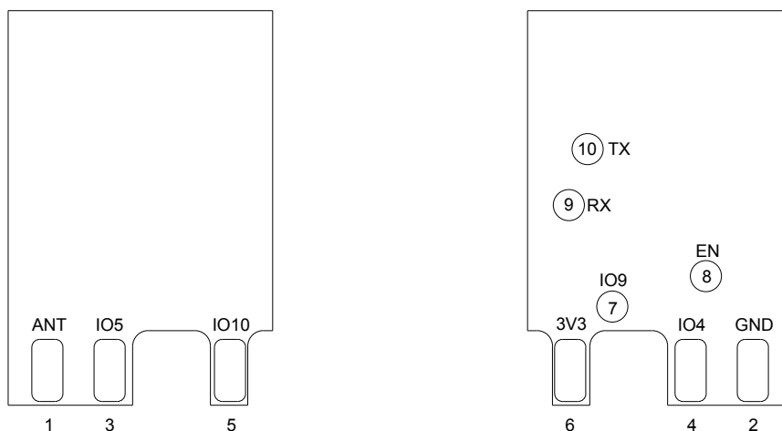
Figure 2: Pin Layout
