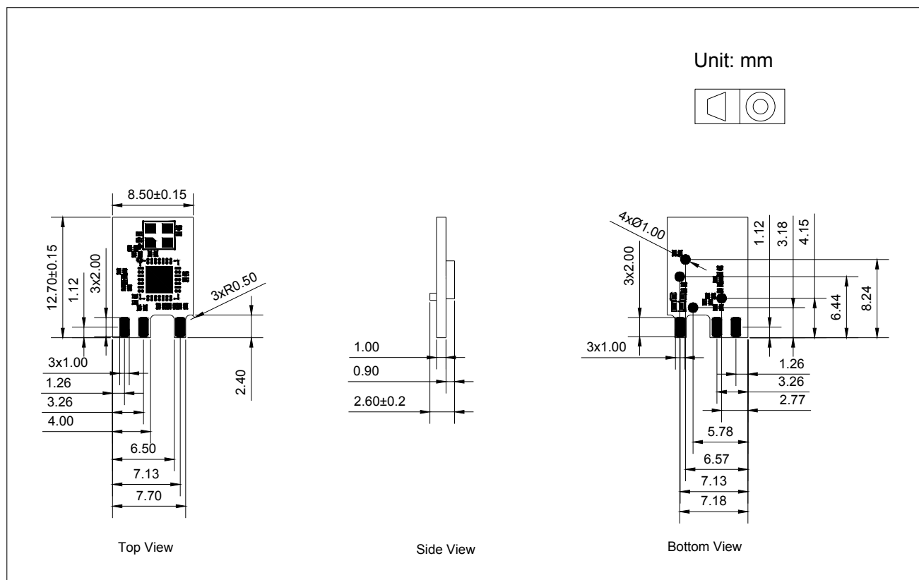
Figure 6: Physical Dimensions
